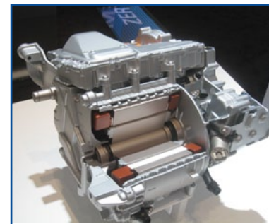
ZF - An all-electric central drive for city buses.
