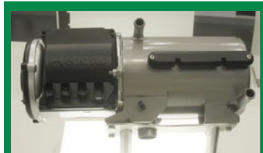
WEBASTO - The new series of water heaters Thermo Top Pro 120 and Thermo Top Pro 150 of 12 and 15 kW and Cool Top 110 RT-CS climate group for mini and midibuses, with 11 kW of cooling capacity and 12 kW of heating capacity.
